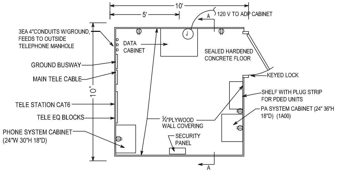
CISIC ROOM FLOOR PLAN (1 DATA CABINET, SMALL STORES)
